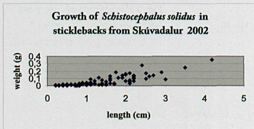
Fig. 6A "Growth" (weight versus length) of plerocercoids of Schistocephalus solidus in sticklebacks from Skúvadalur, 2002.
