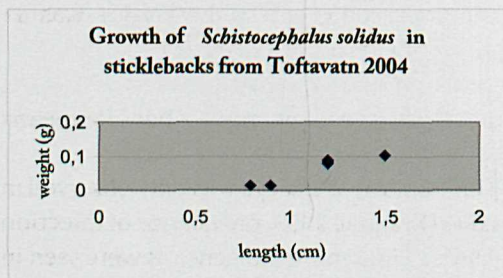
Fig. 6E "Growth" (weight versus length) of plerocercoids of Schistocephalus solidus in sticklebacks from Toftavatn, 2004.
