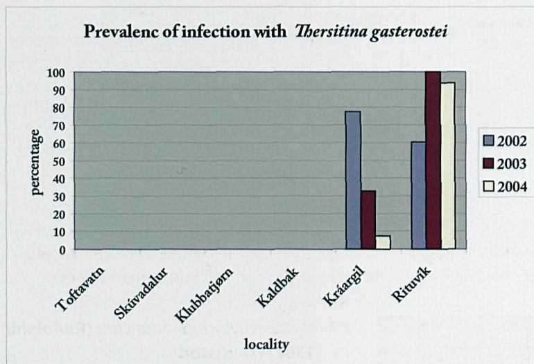
Fig. 3A Prevalence of infection with the Thersitina gasterostei , in sticklebacks from all stations.
