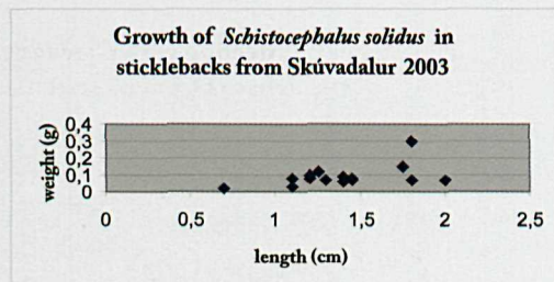
Fig. 6B "Growth" (weight versus length) of plerocercoids of Schistocephalus solidus in sticklebacks from Skúvadalur, 2003.
