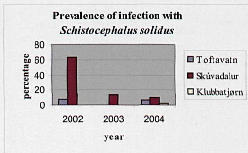
Fig. 5A Prevalence of infection with Schistocephalus solidus , in sticklebacks from all stations.
