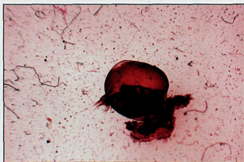
Fig. 4B Micrographs of Thersitina gasterostei (male, quick-stain, x 50)
