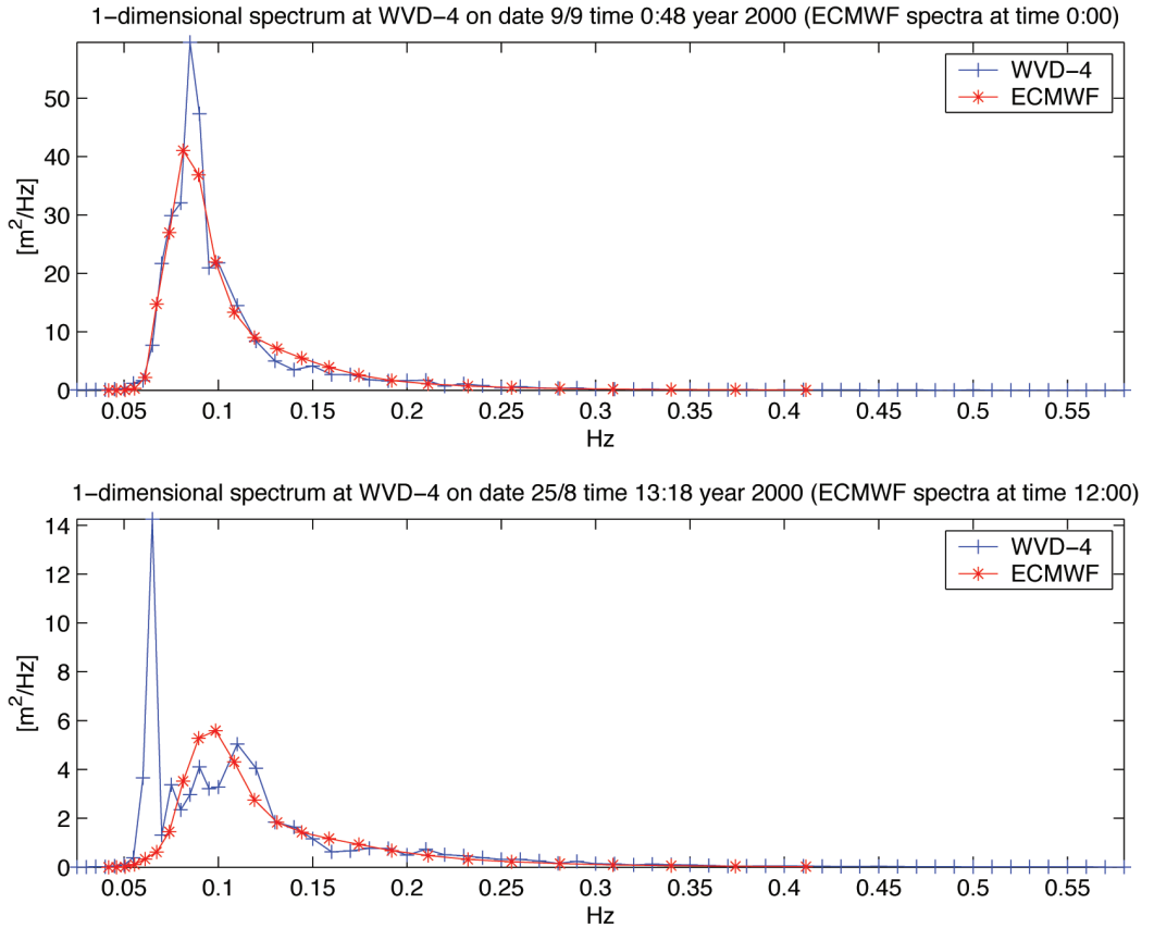
Figure 7. Two recorded 1D wave spectra at WVD-4 in Event 1 vs. 1D-wave spectra from ECMWF.
