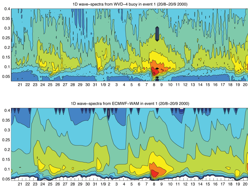
Figure 6. All recorded 1D wave spectra at WVD-4 in Event 1 vs. 1D-wave spectra from ECMWF. y-axis gives frequency, x-axis gives time and colours give the logarithm of the spectral energy density. The spurious spectral feature occurring in the WVD-4 spectra on the 8/9 is due to data error.
