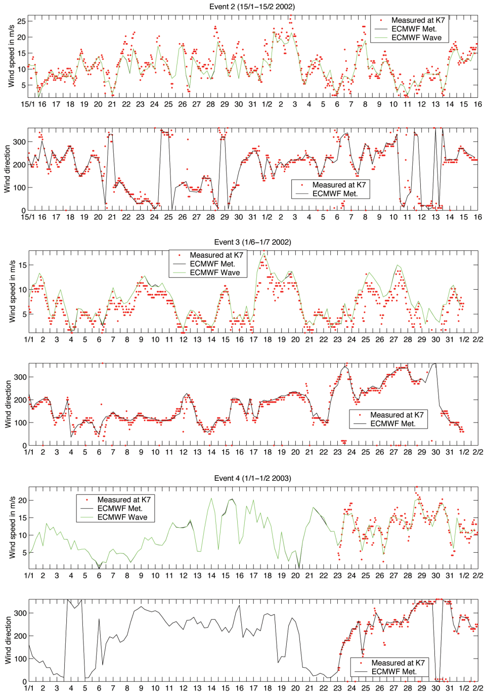
Figure 2. The recorded and predicted wind speed and direction at the MetOffice K7 station for the second, third, and fourth hindcasted periods respectively. Note that the wind observations are not adjusted to 10m.
