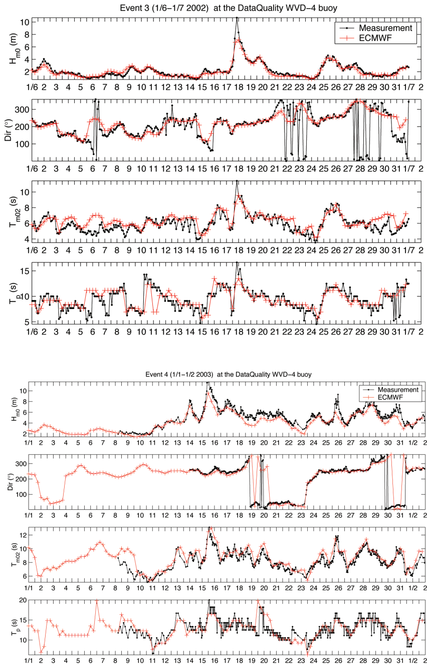
Figure 5. Recorded and predicted wave parameters H_{m0} , Dir , T_{m02} and T_p at location WVD-4, for Event 3 and 4 respectively.
