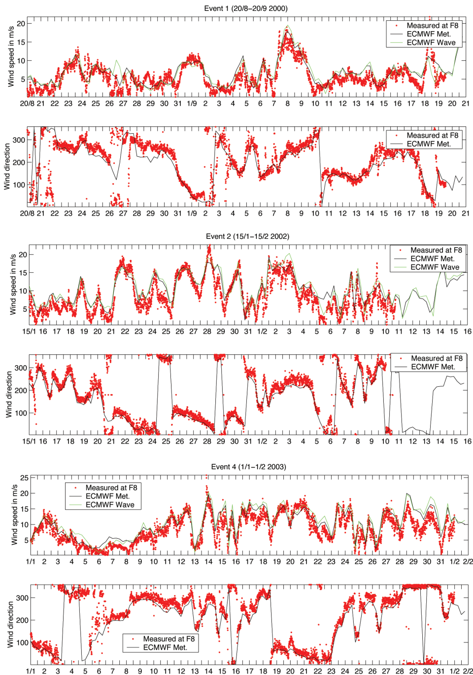
Figure 3. The recorded and predicted wind speed and direction at the Glyvursnes F8 station for the first, second, and fourth hindcasted periods respectively.
