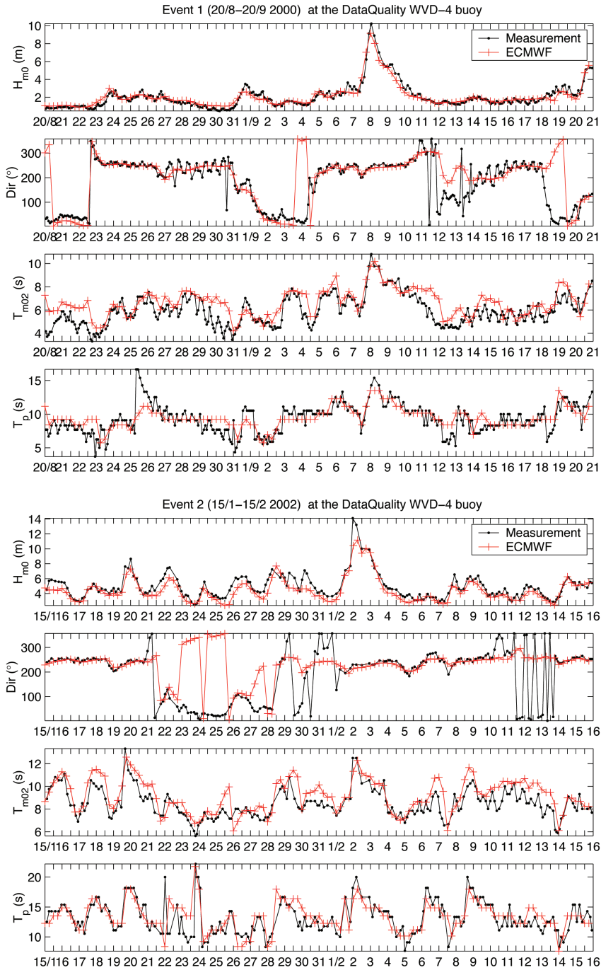
Figure 4. Recorded and predicted wave parameters H_{m0} , Dir , T_{m02} and T_p at location WVD-4, for Event 1 and 2 respectively.
